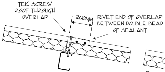
End Lap Detail
