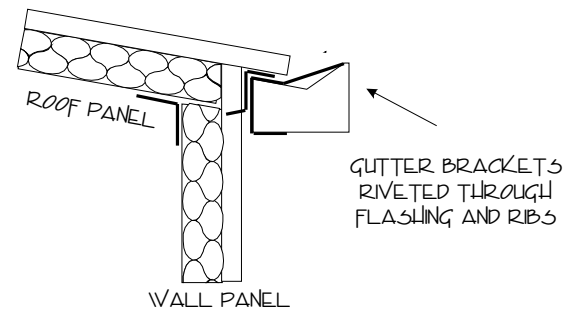
Gutter Detail
