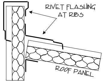
Lean To Roof with Parapet Wall
